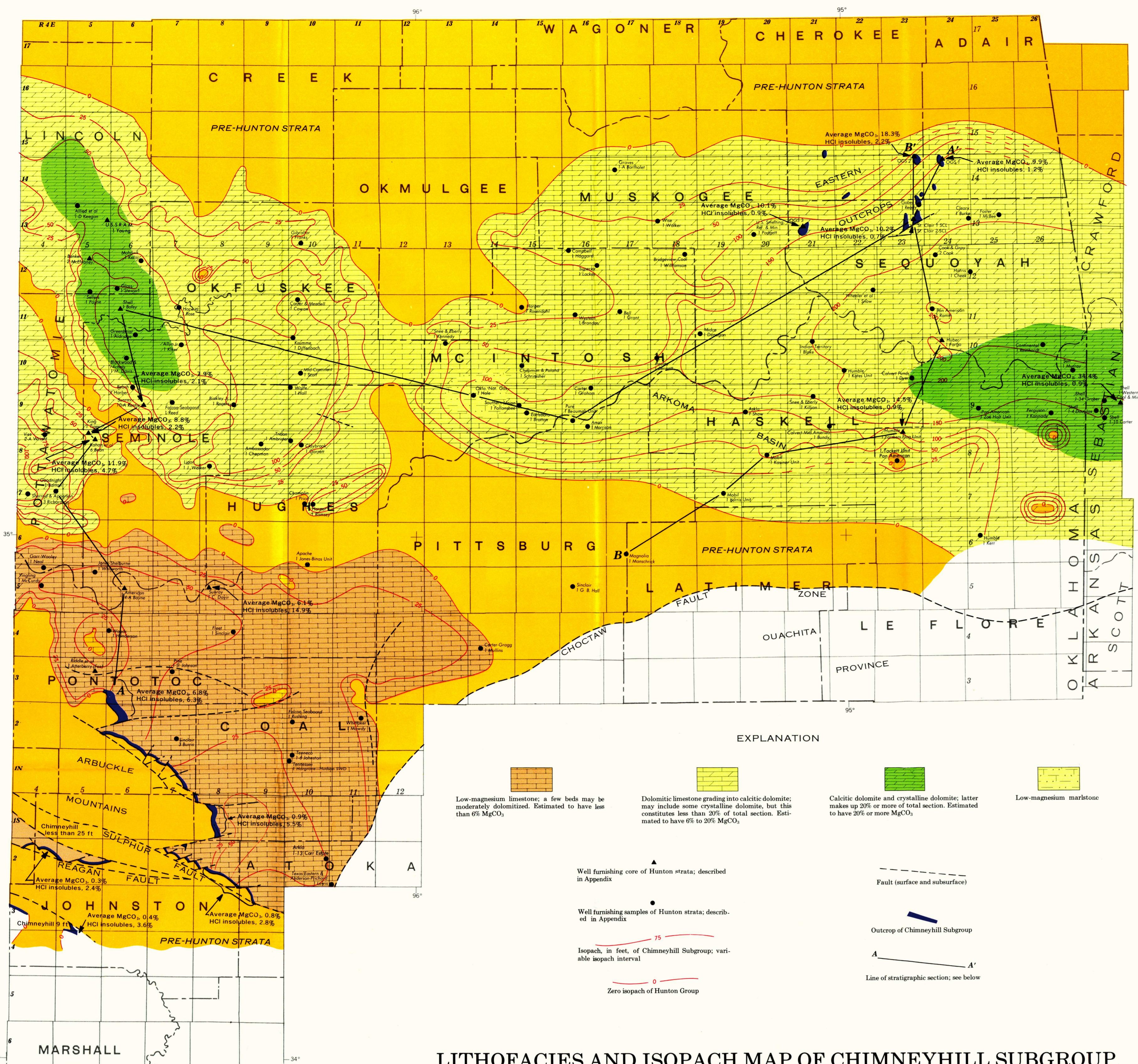
LITHOFACIES AND ISOPACH MAP OF CHIMNEYHILL SUBGROUP IN EASTERN OKLAHOMA
