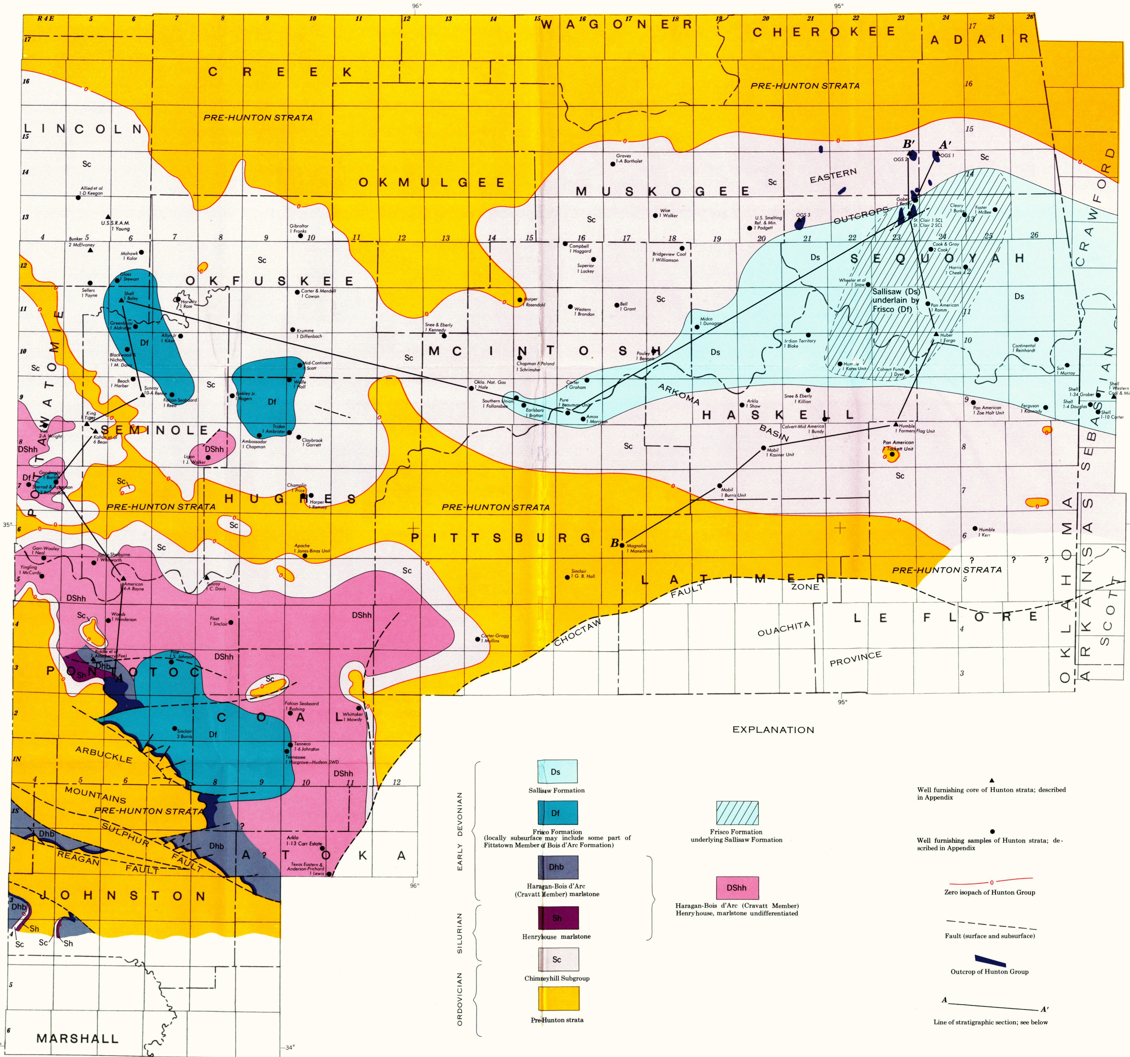
PRE-WOODFORD GEOLOGIC MAP IN EASTERN OKLAHOMA
