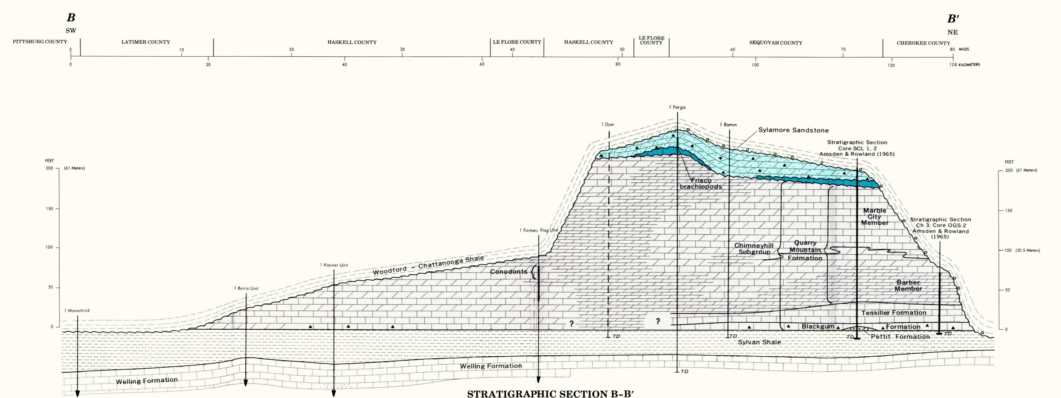
STRATIGRAPHIC SECTION B-B'
