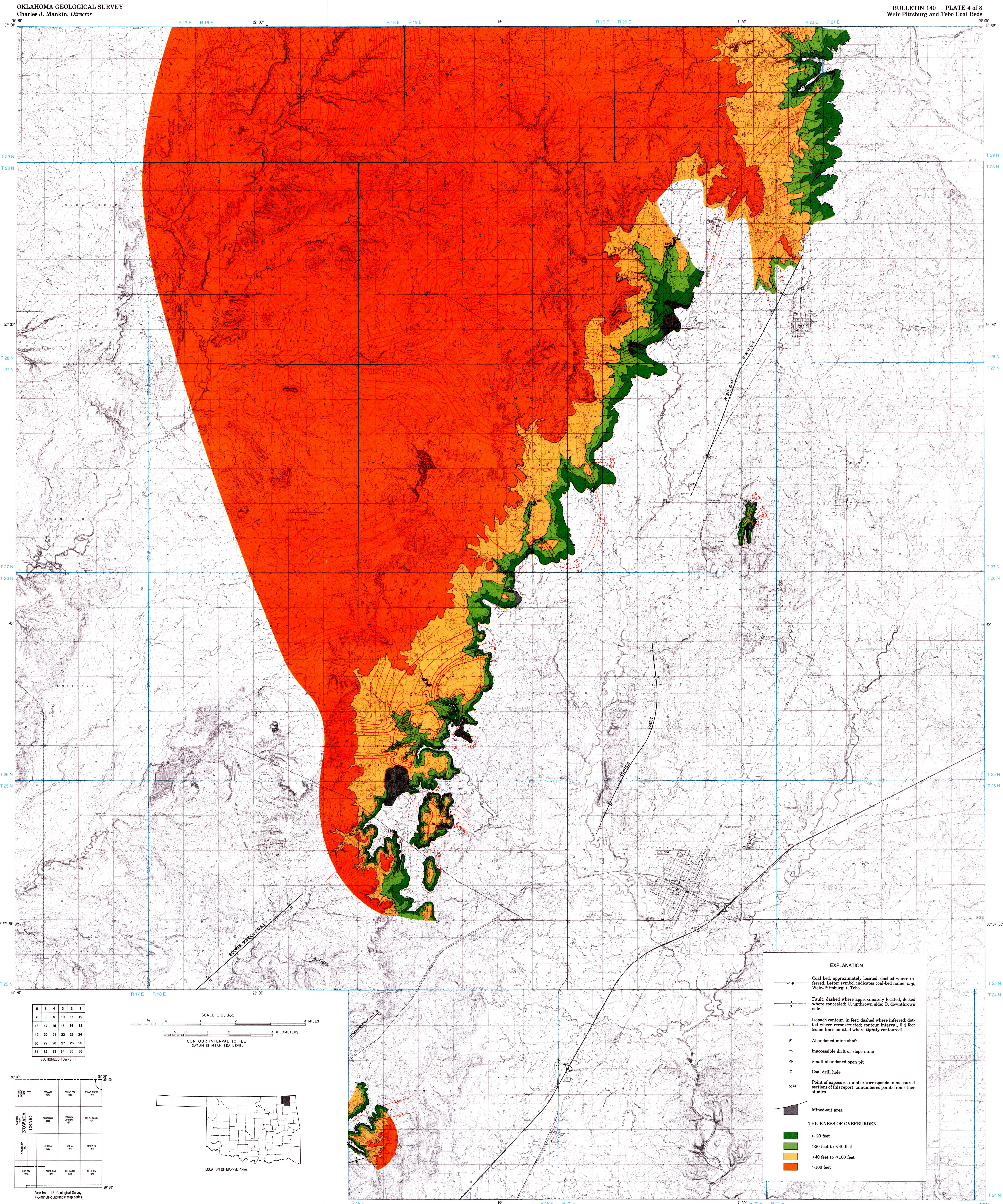
MAP OF WEIR-PITTSBURG COAL BED IN CRAIG AND EASTERN NOWATA COUNTIES, OKLAHOMA (Includes Data for Tebo Coal)
