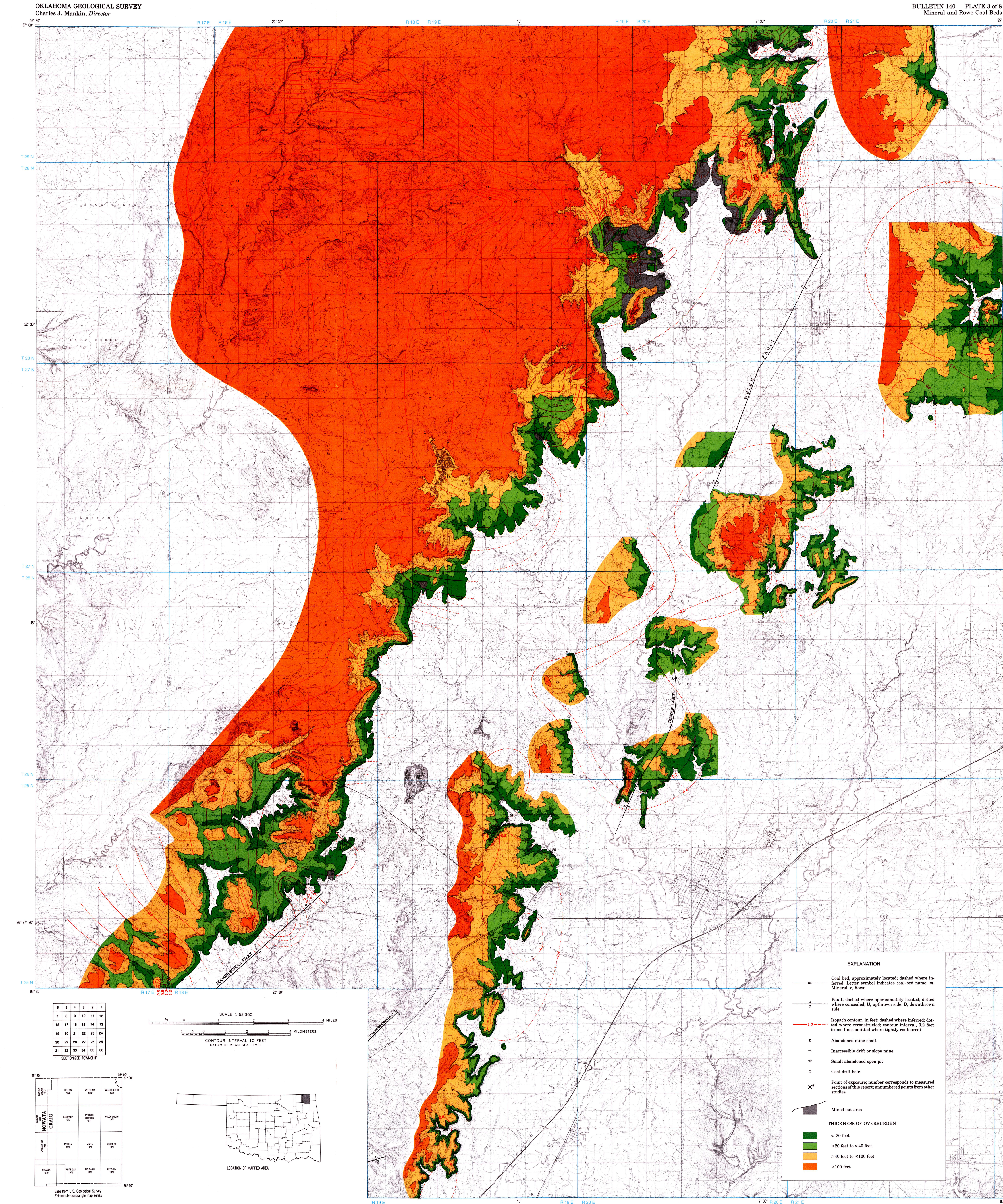
MAP OF MINERAL AND ROWE COAL BEDS IN CRAIG AND EASTERN NOWATA COUNTIES, OKLAHOMA
