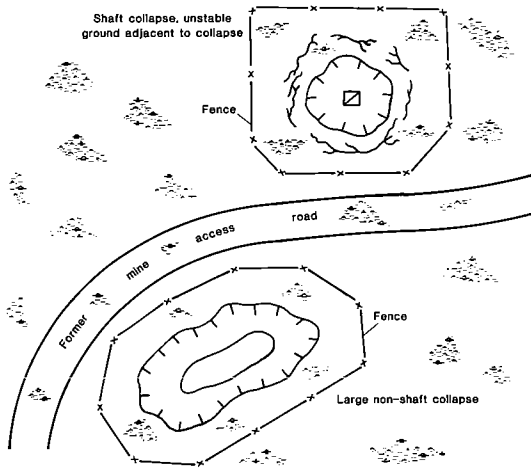
Figure 17. Fencing is a suggested safeguard for shaft collapses with adjacent unstable ground, as well as for very large collapse features. Periodic surveillance and maintenance of fences would be required.
