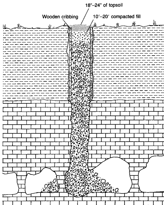
Figure 15. Schematic cross section of open mine shaft, illustrating one way to seal or close the opening in early stage of shaft failure.
