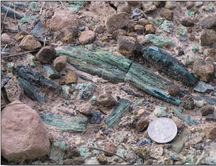
Figure 9. Malachite- and azurite-coated wood from near the base of the Matfield Shale (Wolfcampian), near Pawnee.
