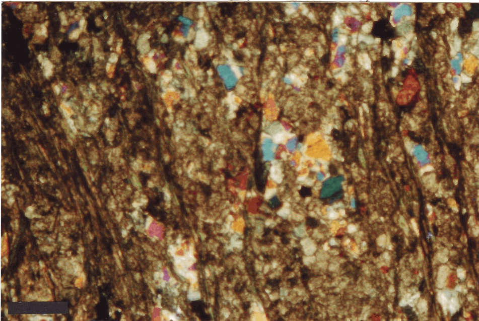
PLATE 265: Sandy meta-dolomite cut by numerous thin mica filled stylolites. 12,137'.
