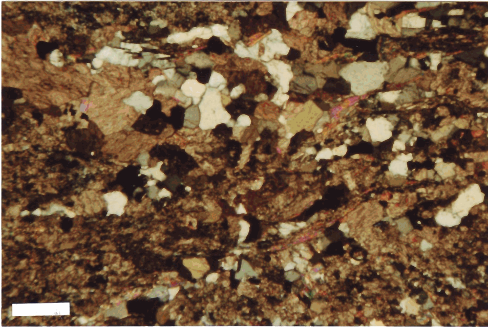
PLATE 264: Sandy meta-dolomite cut by numerous thin mica filled stylolites. 12,137'.
